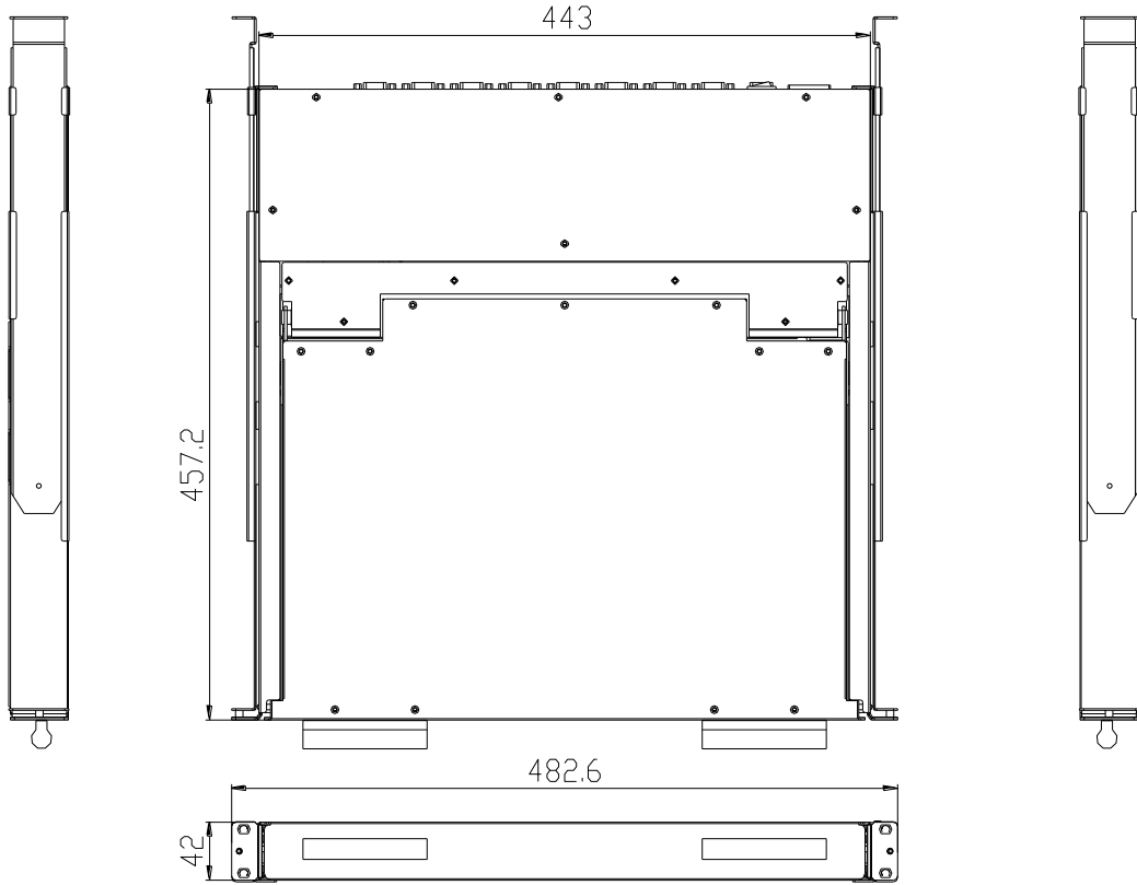
Rear of KVM-1701SW-AST-M2
